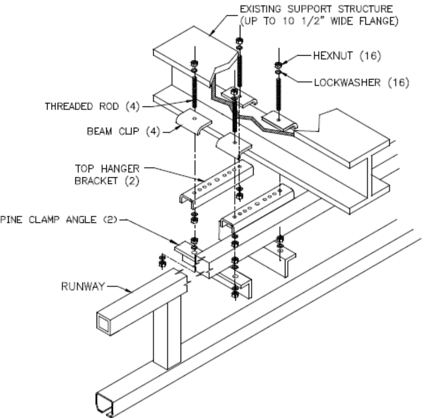
Trussed track with 1-1/2" to 2-1/2" top tube.
